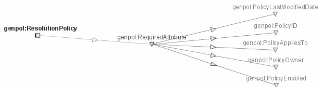
Figure 15. Resolution Policy Attributes
