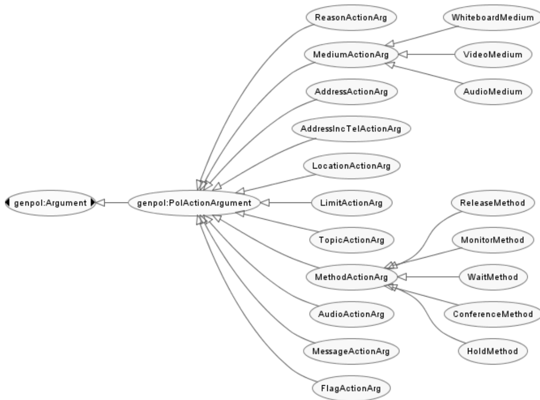
Figure 19. Call Control Action Arguments
