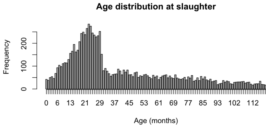
Figure 23: Age distributions of beef herds in GB in 2006 used to determine the age structure for the model. The age of the animals at the time of test (top) is calculated as the proportion of all tests that either test positive or clear, inconclusives are ignored. The age distribution at slaughter (bottom) is obtained from the age of the animals when presented at slaughter.
